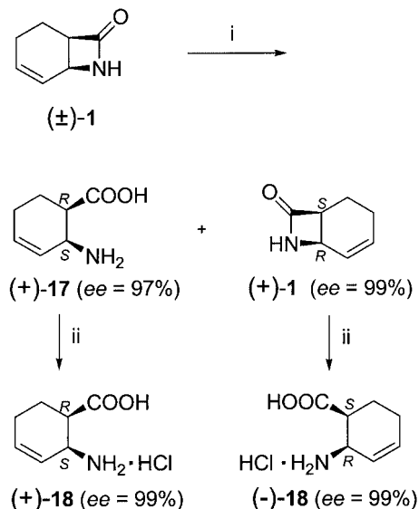
Scheme 4. Reagents and conditions: (i) CAL-B, H 2 O (1 equiv.), i Pr 2 O, 65 °C; (ii) 18% HCl.
