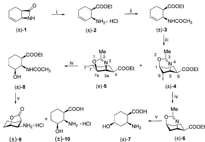
Scheme 1. Reagents and conditions: (i) 12% HCl, EtOH, reflux, 2 h, 76%; (ii) MeCOCl, Et 3 N, CHCl 3 , room temp., 2 h, 98%; (iii) NaI, I 2 , NaHCO 3 , CH 2 Cl 2 , 0 °C, 20 h, 4 : 27%, 5 : 63%; (iv) Bu 3 SnH, AIBN, toluene, 60 °C, 6 h, N 2 , followed by chromatography, 6 : 65%, 8 : 58%; (v) 10% HCl, H 2 O, reflux, 30 h, 7 : 88%, a mixture (1:2) of 9 and 10 : 85%.
