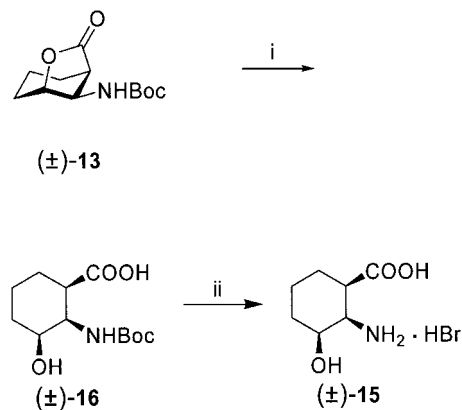
Scheme 3. Reagents and conditions: (i) LiOH, H 2 O, THF, room temp., 5 h, 98%; (ii) Me 3 SiBr, phenol, CH 2 Cl 2 , room temp., 2 h, Ar atmosphere, 76%.
