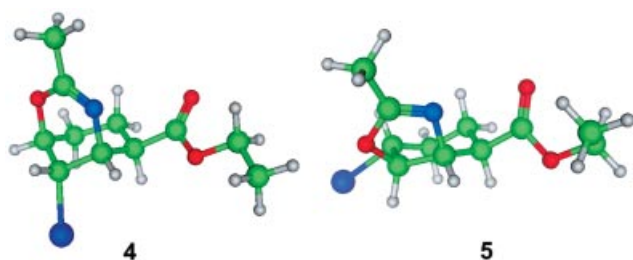
Figure 2. Stereoviews of typical minimum-energy structures of 4 and 5 .
