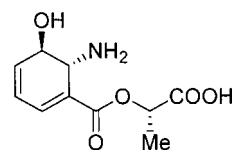
Figure 1. The structure of oryzoxymycin.
