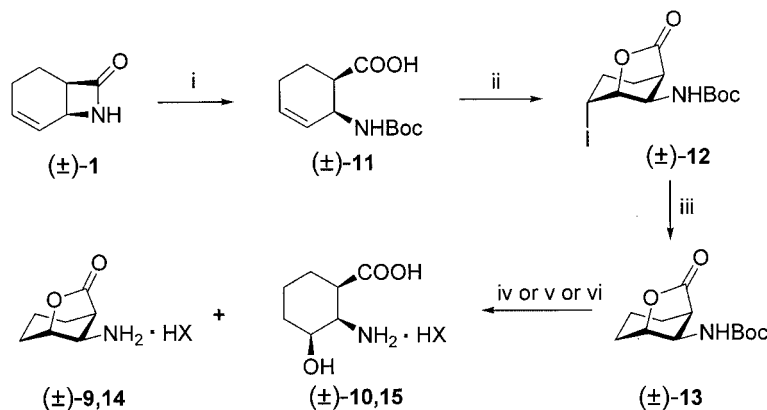
Scheme 2. Reagents and conditions: (i) Boc 2 O, Et 3 N, DMAP, THF, room temp., 3 h, then LiOH, H 2 O/THF, room temp., 5 h, 90%; (ii) I 2 , NaI, NaHCO 3 , CH 2 Cl 2 , 0 °C, 20 h, 91%; (iii) Bu 3 SnH, AIBN, toluene, 60 °C, 20 h, N 2 , 98%; (iv) HCl/H 2 O, room temp., 12 h; (v) HBr/H 2 O, room temp., 12 h; (vi) Me 3 SiBr, phenol, CH 2 Cl 2 , room temp., Ar, 2 h, 65%; 9 and 10 : X = Cl; 14 and 15 : X = Br.
